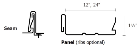
A1500 1 1/2" Snap-Lock
