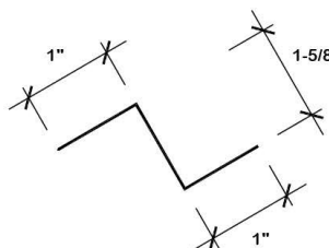
Z-Closure Flashing (Closed or Vented)
