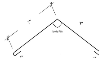
Hip & Ridge Flashing
