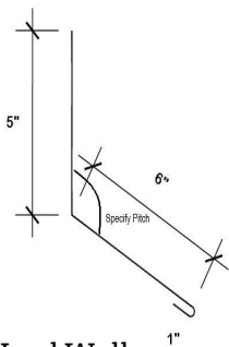
Head Wall Flashing
