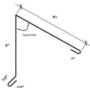
Peak Flashing
